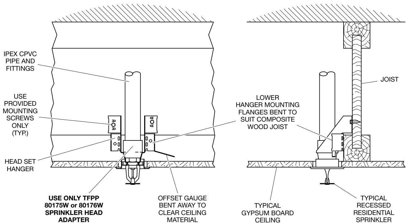
FIGURE 2 SIDE-MOUNT INSTALLATION OF HANGER HEAD SET PROVIDING ACCURATE VERTICAL POSITIONING OF THE SPRINKLER
