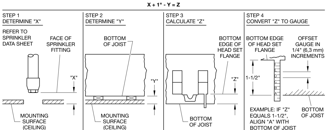
FIGURE 3 USE OF OFFSET GAUGE FOR HANGER HEAD SET
