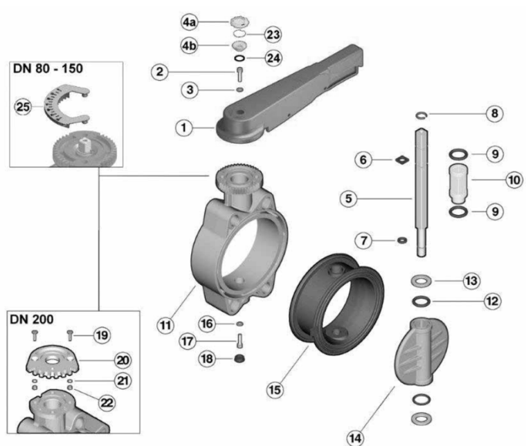
Sizes 2-1/2" to 8"
