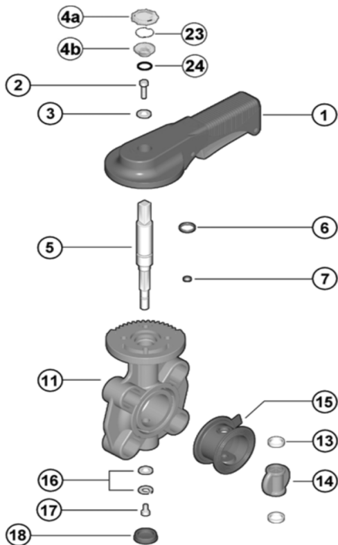
Sizes 1-1/2" to 2"
