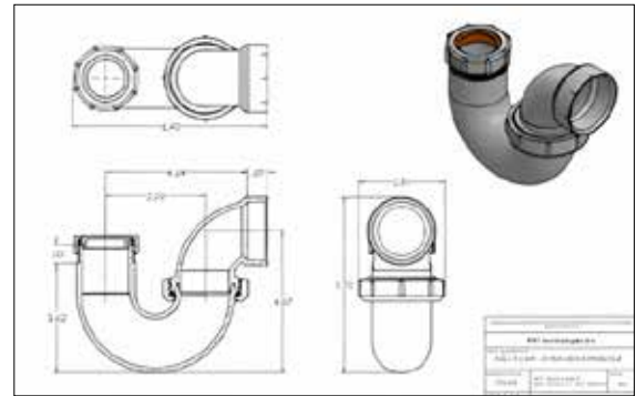
Dimensional Drawings
