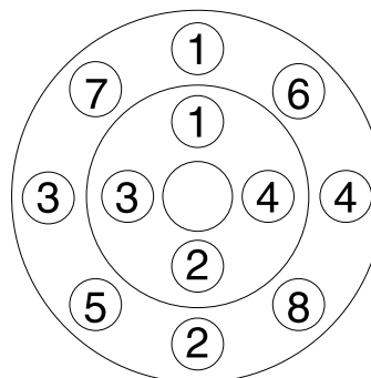
Flange Bolt Tightening Patterns
