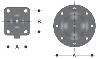
Sizes 3"
