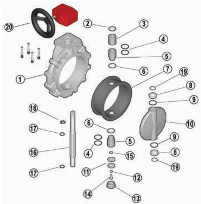
Size 10" – 12"
