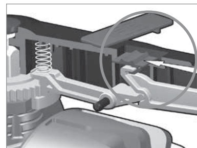
LOCK
