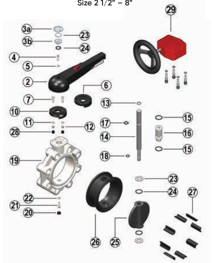
Size 2 1/2" – 8"
