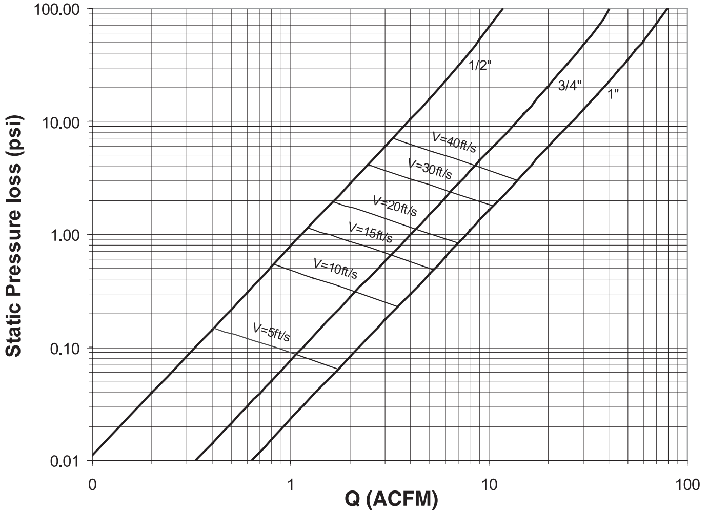
Figure B6 Pressure Loss per 100 Feet of Duratec Pipe Air at 160 psig (174.7 psia), 60°F
