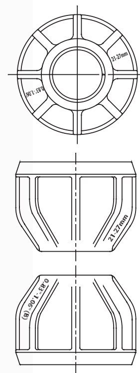
Philmac Universal Transition Coupling 0.9" – 1.0" OD (21mm – 27mm OD)
