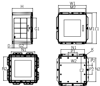
JBX12124 - JBX161610
