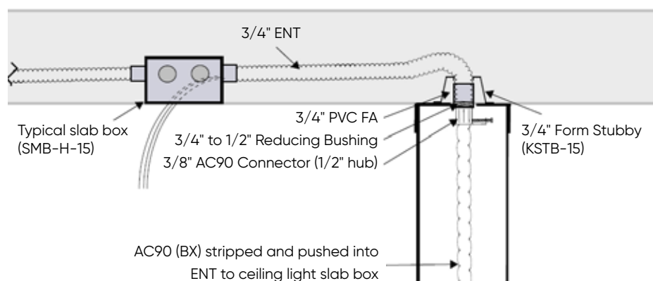
Typical Suspended Slab
